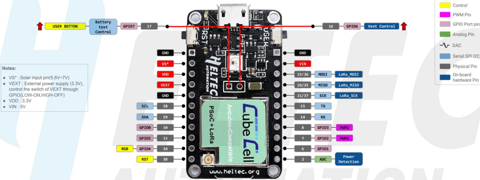
CubeCell HTCC-AB01 Pinout Diagram
