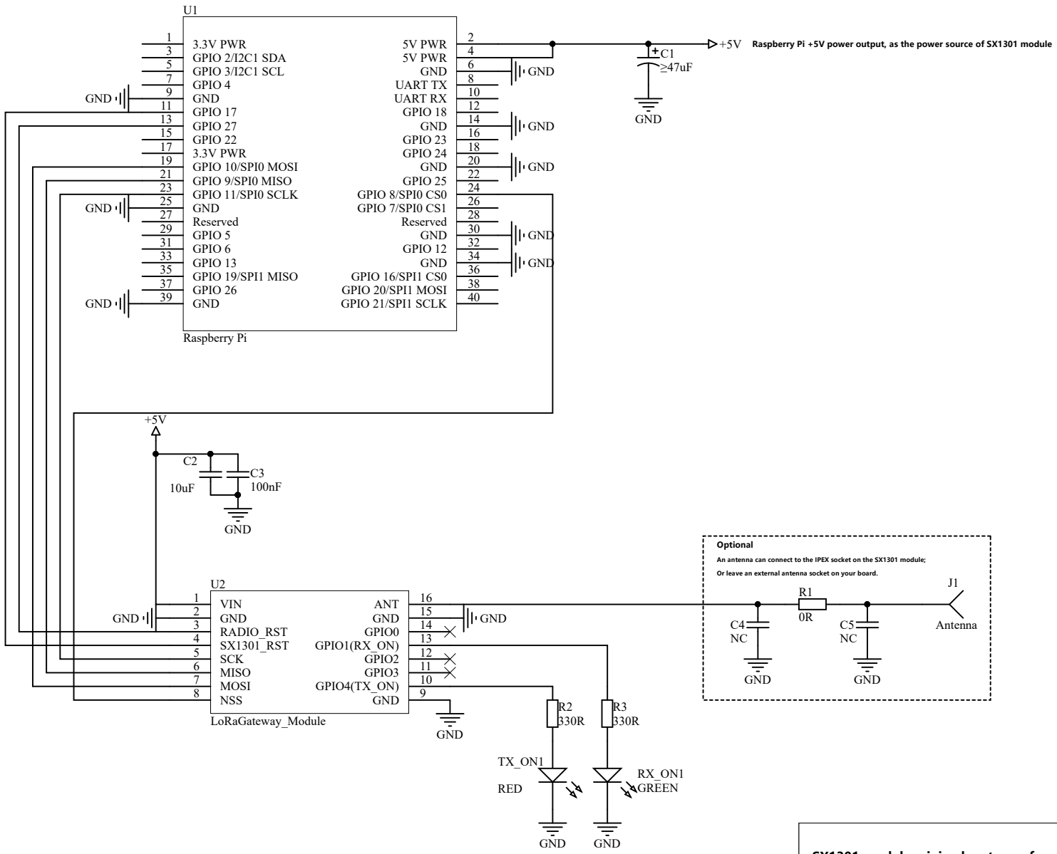
SX1301 module minimal system reference design
